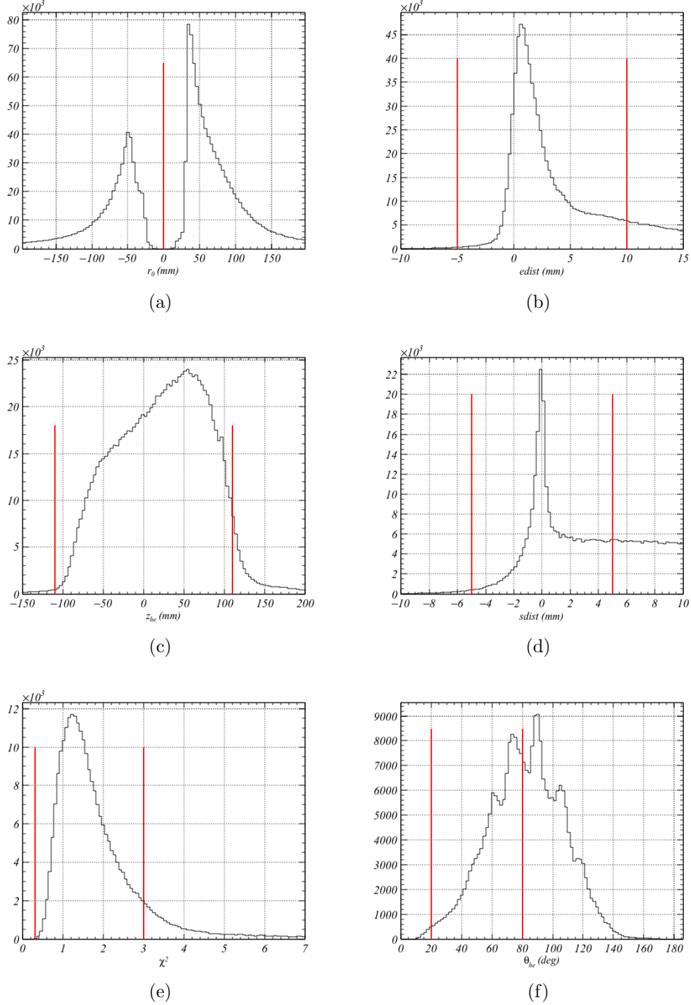
FIG. 36: Summary of the cuts on RTPC variables to select helium-4. (a) The curvature of the path. (b) The closest ionization point to the anode. (c) Vertex of the tracks. (d) The closest ionization point to the cathode. (e) Fit quality cut. (f) Cut on the polar angle of the track.
