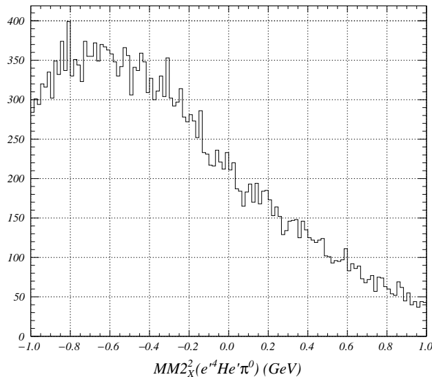
FIG. 58: Missing mass MM^2_X(e'^4He'\pi^0) spectrum for EC-IC combination.
