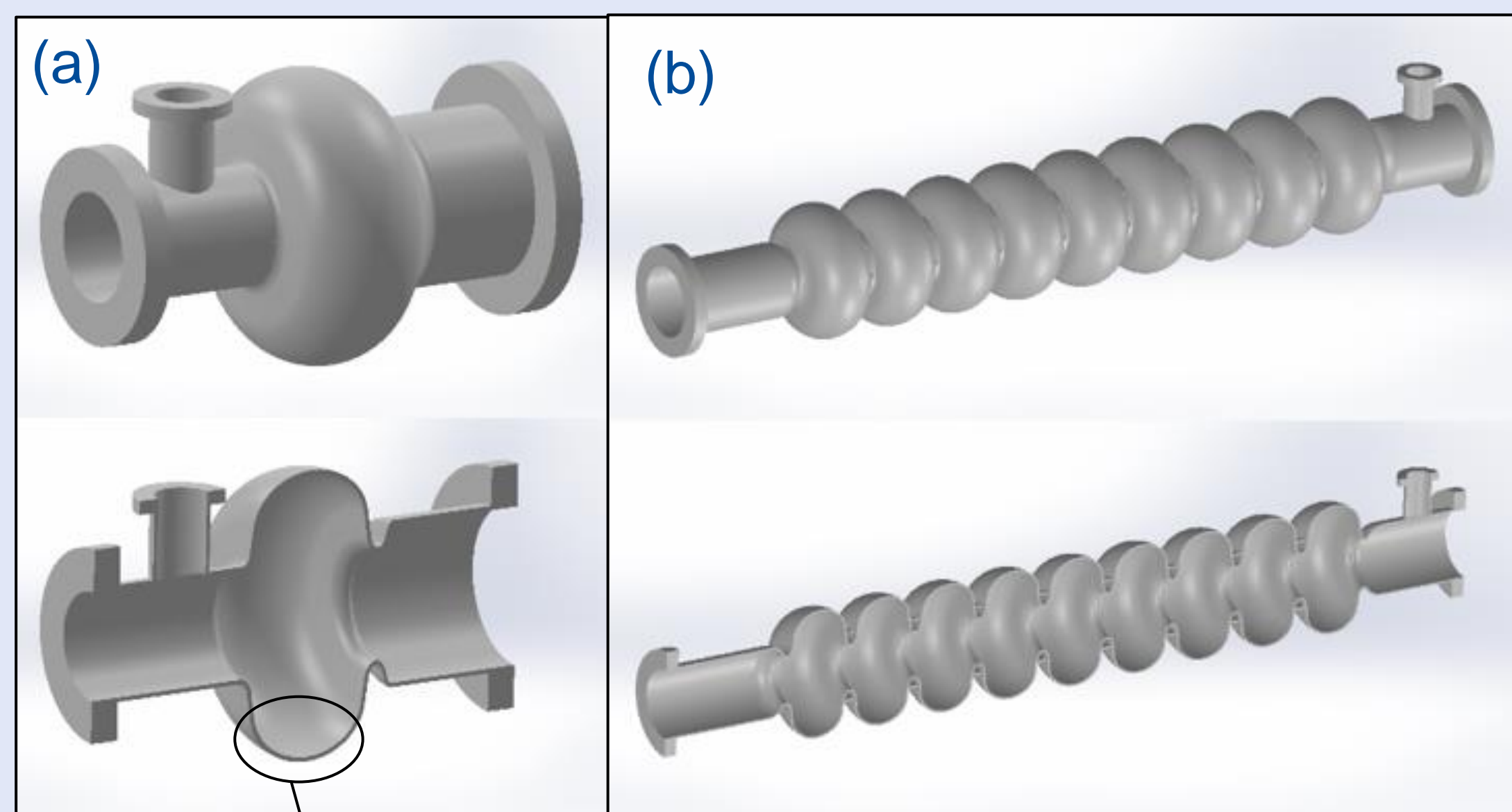
Niobium SRF Cavity (a) single cell (b) 9-cell
