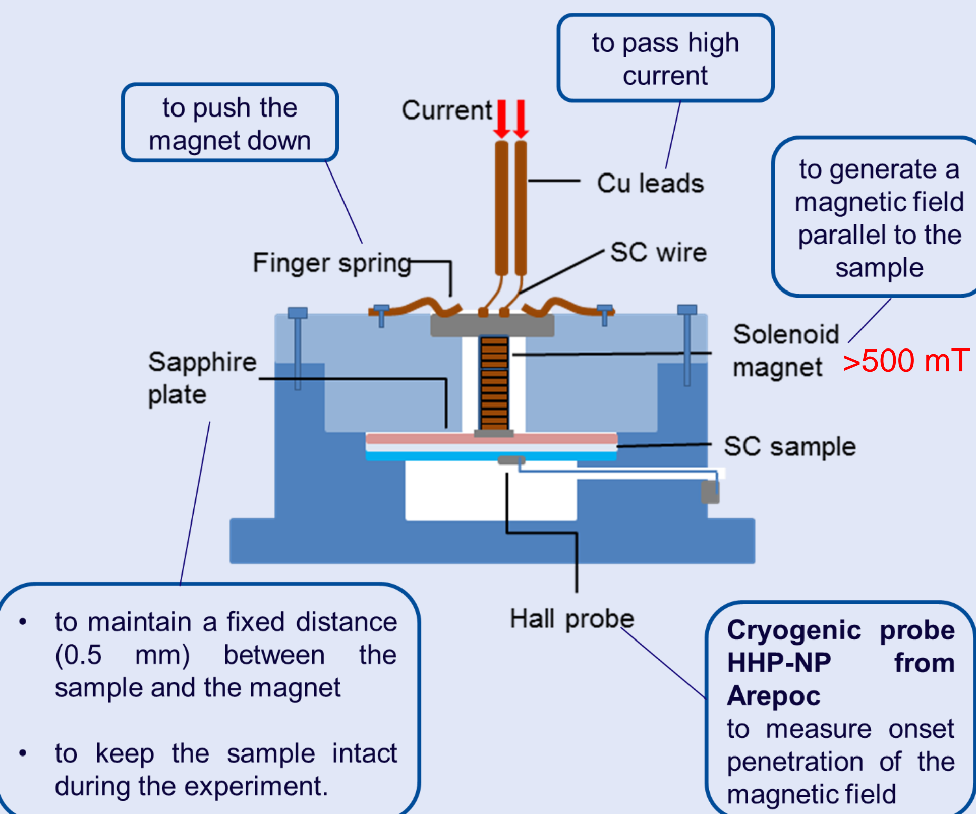
Schematic cross section of detailed experimental setup
