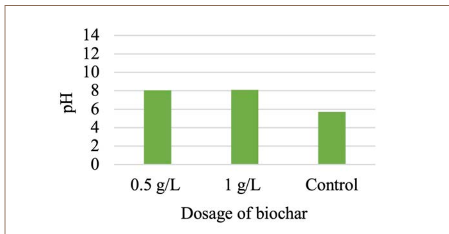
Figure 4 — Change in pH after adding biochar in the reactor concentration = 10 mg/L
