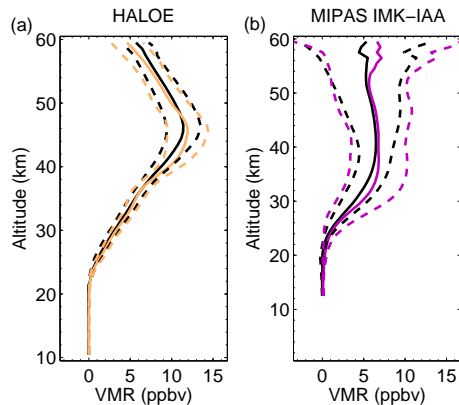
Figure 3. Mean NO profiles (in ppbv) for coincident diurnally scaled ACE-FTS (black) and HALOE (left panel) and MIPAS IMK-IAA (right panel) measurements and corresponding measurement standard deviations (dashed lines). Coincidence criteria for HALOE comparisons are within 3 h and 500 km and are within 3 h and 100 km for MIPAS IMK-IAA comparisons.
