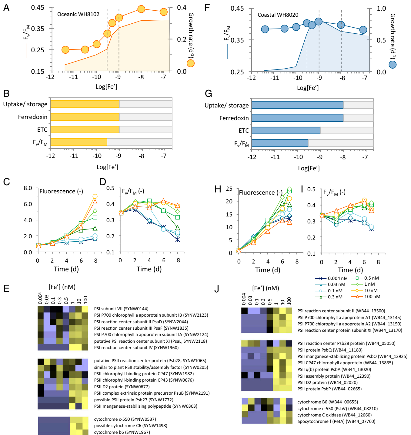
Fig. 2. Physiological and photosynthetic responses of oceanic WH8102 (Left, A–E) and coastal WH8020 (Right, F–J) to [Fe'] . Vertical dashed lines in A and F and bars in B and G indicate the concentration of Fe' (plotted as \log[Fe'] ) at which a given physiological parameter showed a threshold response (Materials and Methods). Growth rate (circles) and photosynthetic efficiency ( F_v/F_M ) measured at the time the protein samples were collected, shaded regions are shown in A and F. ETC, membrane proteins in the photosynthetic electron transport chain. Growth curves are shown in C and H and photosynthetic efficiency ( F_v/F_M ) values collected each day are shown in D and I. Legend for C, D, H, and I is shown below I. (E and J) Heatmap of photosynthetic electron transport chain proteins for Synechococcus sp. strains WH8102 (E) and WH8020 (J). Normalized spectral counts are given in SI Appendix, Table S4. Color indicates higher (yellow) or lower (purple) abundance relative to the centered mean value (black).
