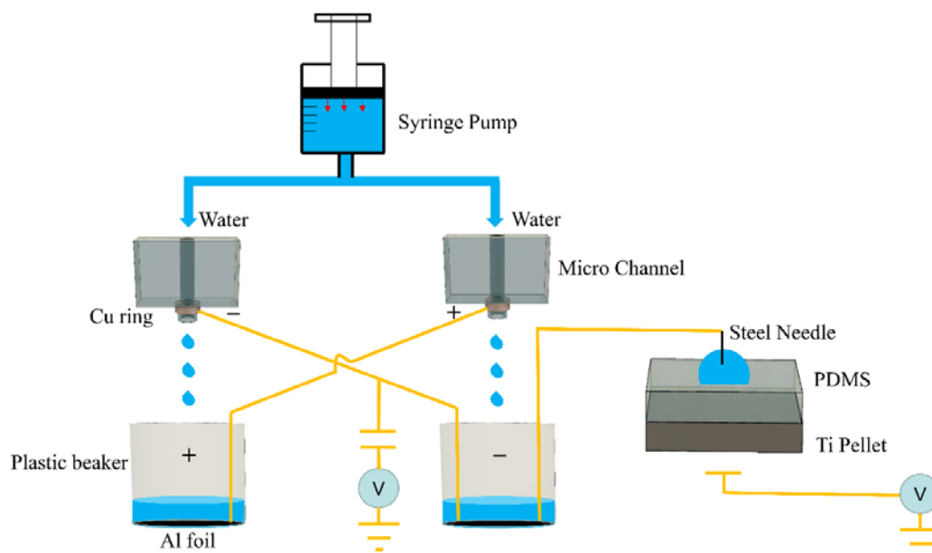
Figure 1. Schematic diagram of the electrowetting system using the microfluidic Kelvin water dropper (MKWD).
