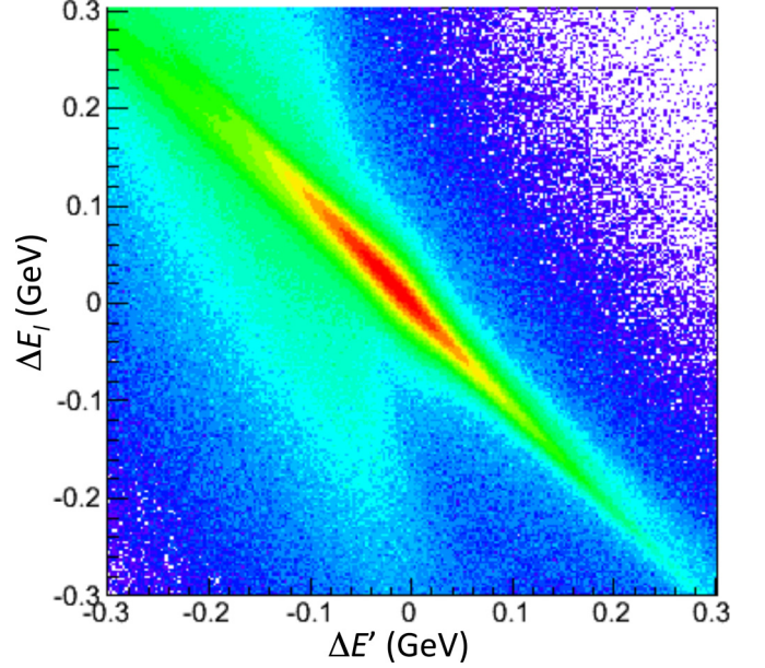
FIG. 14. \Delta E_l and \Delta E' distributions for candidate e^- p events prior to application of kinematic cuts showing the linear correlation between \Delta E_l vs \Delta E' . An identical correlation is seen for e^+ p events.
