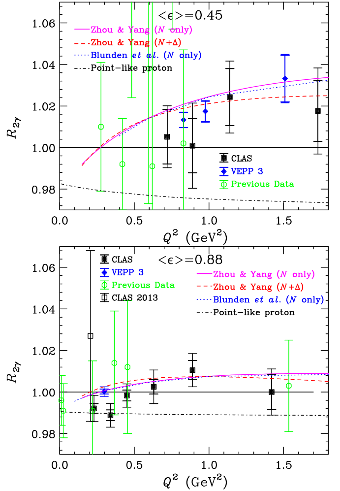
FIG. 21. Same as Fig. 20 except as a function of Q^2 at \epsilon \approx 0.45 (top) and 0.88 (bottom). Also included is the CLAS 2013 [38] result (black open square), which has been averaged to a single point at \epsilon = 0.893 . The open green circles show the previous world data at 0.2 \leq \epsilon \leq 0.7 and 0.7 \leq \epsilon \leq 0.95 in the top and bottom plots, respectively [32].
