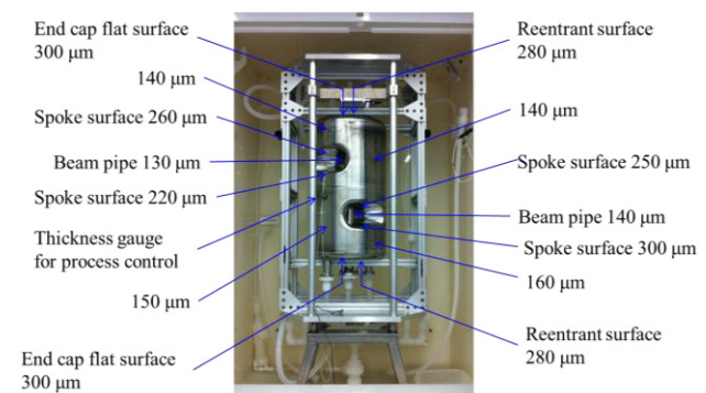
Figure 6: BCP set-up and thickness measurement results.
