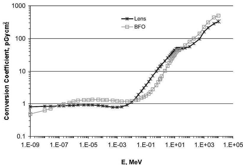
Fig. 1. Neutron dose conversion factors for ocular lens and BFO.
