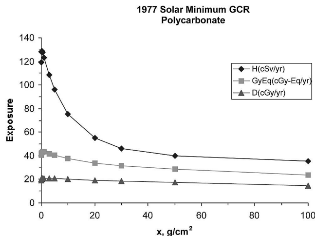
Fig. 3. Attenuation of dosimetric quantities within polycarbonate shield of thickness x .
