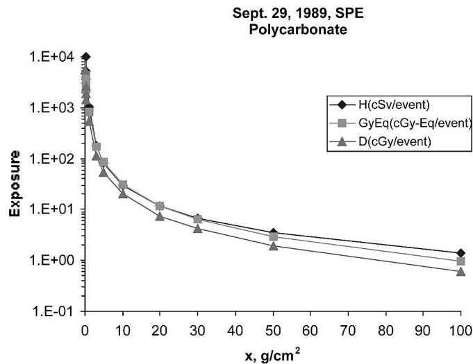
Fig. 2. Attenuation of dosimetric quantities within polycarbonate shield of thickness x .
