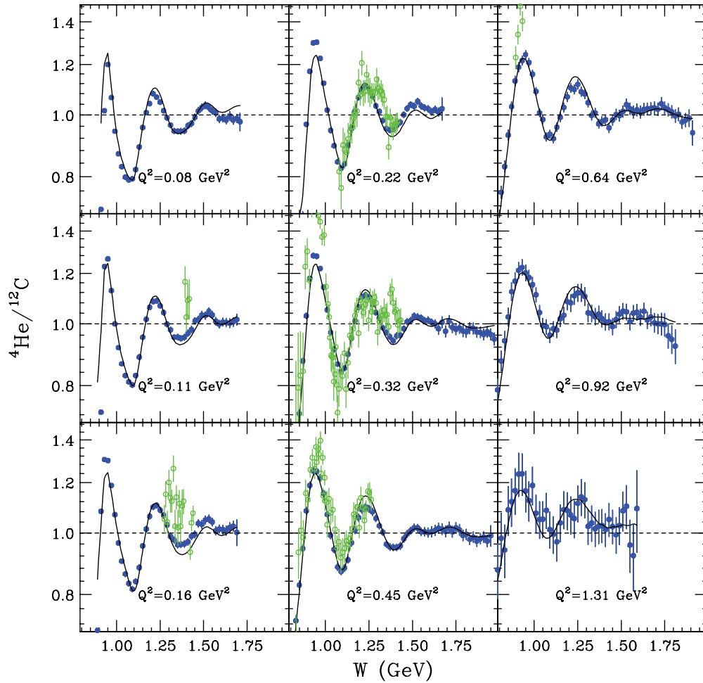
FIG. 1. (Color online) Extracted ratios of ^4\text{He} to ^{12}\text{C} cross sections (per nucleon) from this experiment (solid blue circles), using beam energies of 1.6 to 2.2 GeV, showing statistical and point-to-point systematic errors added in quadrature. The overall normalization error is 4%. The solid curves show the ratio of model cross sections. The green open circles are from SLAC Experiment NE5 [18].
