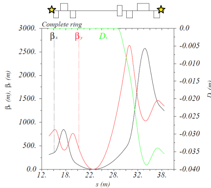
Figure 2: Interaction region optics, where the yellow stars represent the crab cavity locations.
