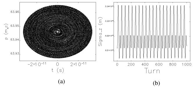
Figure 3: Longitudinal phase space, plotted for the last 20 of a 1000 turns without crab cavities (a), and longitudinal beam size showing oscillations in the order of the numerical errors (b).
