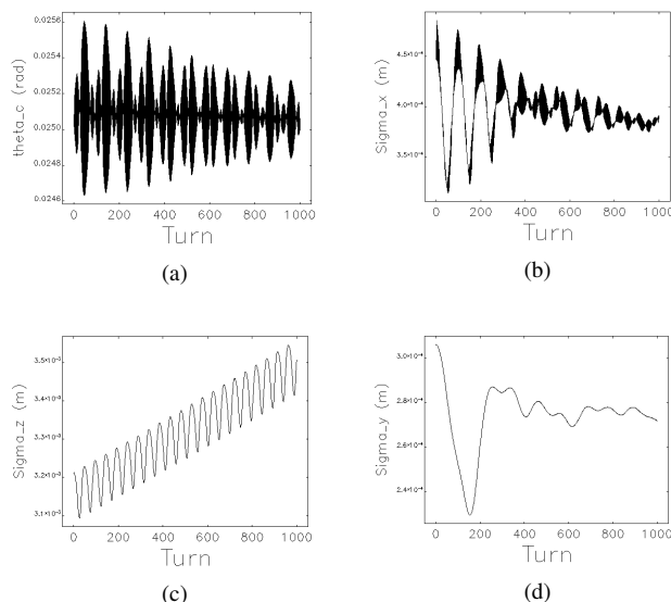
Figure 6: For the case of a small sextupole contribution: the crabbed angle at IP (a), the longitudinal beam size (growing at similar rate than for the pure dipole case) (c), and both horizontal and vertical beam sizes (b) and (d), respectively.
