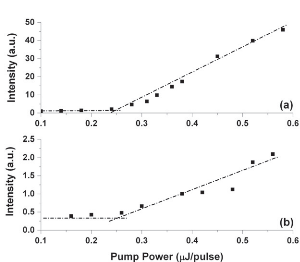
Figure 2. Micro-ring emission intensity as a function of pump power for excitation normal to the minor (a) and major (b) ellipse axes. Dashed lines are only a guide-to-the-eye for approximating the lasing threshold.
