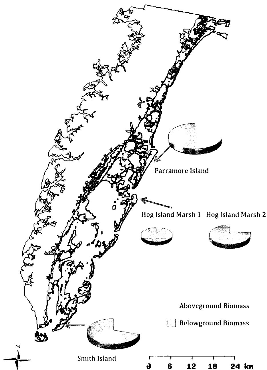
Figure 11. Interisland variation of above and belowground marsh biomass.
