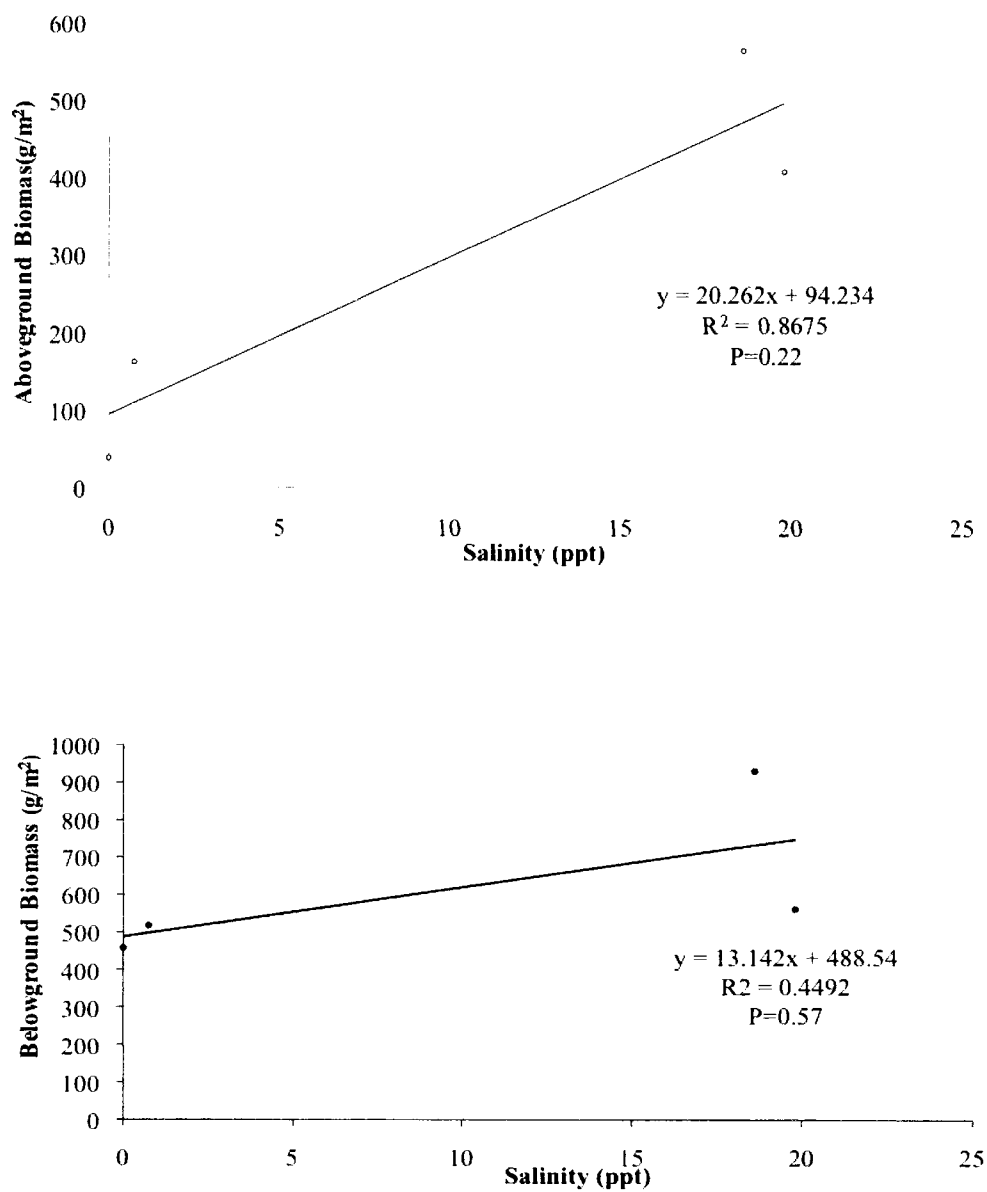
Figure 9. Correlation results for water table salinity of marshes and above and belowground biomass of marshes.
