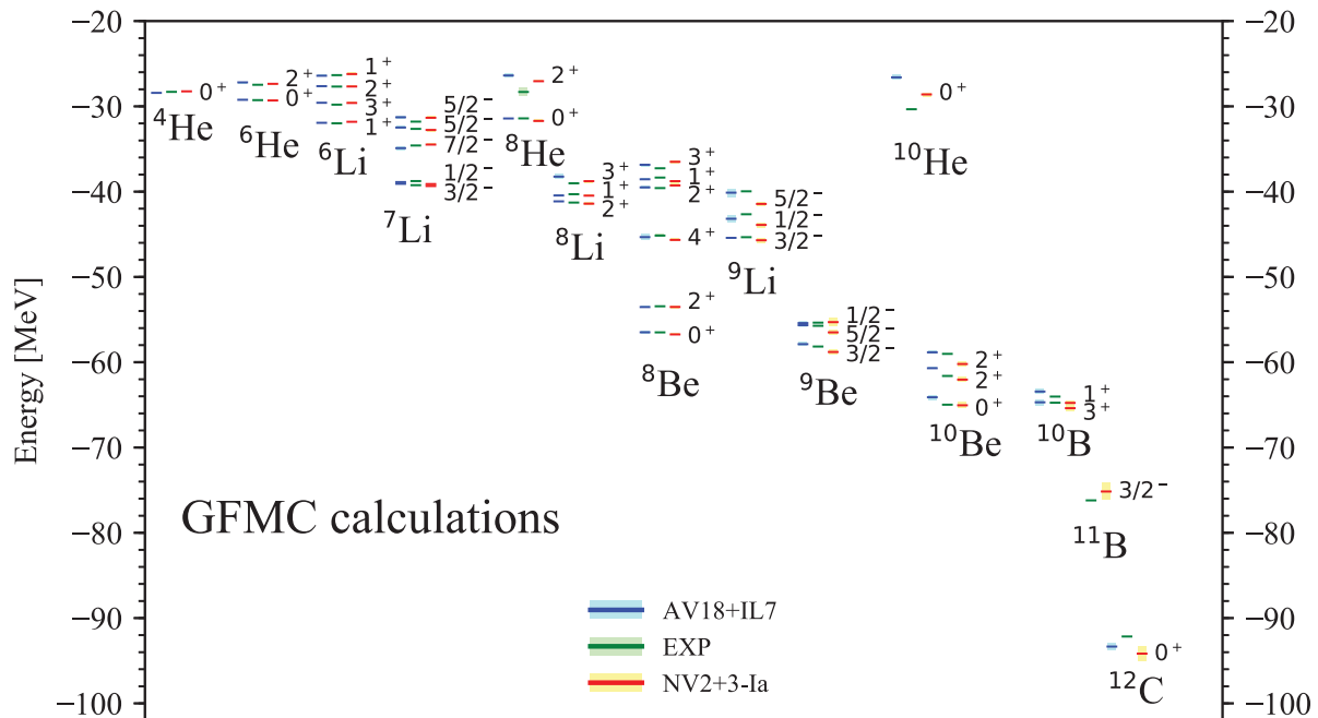
FIG. 2. The energy spectra of A = 4 – 12 nuclei obtained with the NV2 + 3-Ia chiral interactions are compared to experimental data [54]. Also shown are results obtained with the phenomenological AV18 + IL7 interactions [1].
