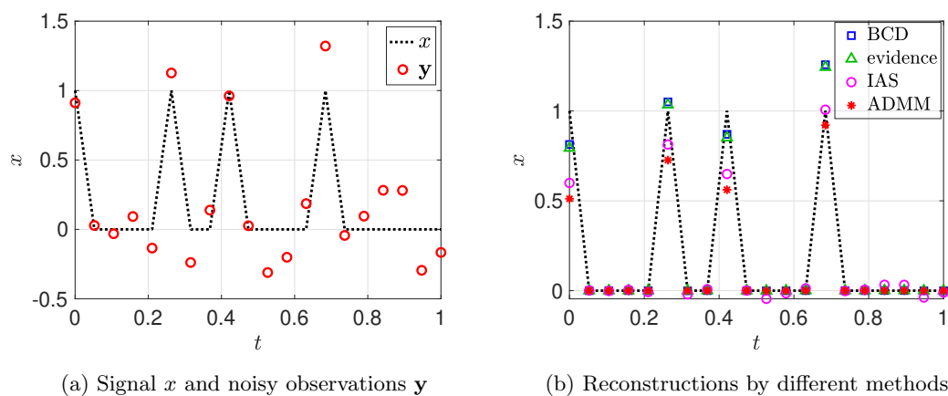
Figure 2. The sparse signal x and noisy observations y at n = 20 equidistant points, and reconstructions by different methods.
