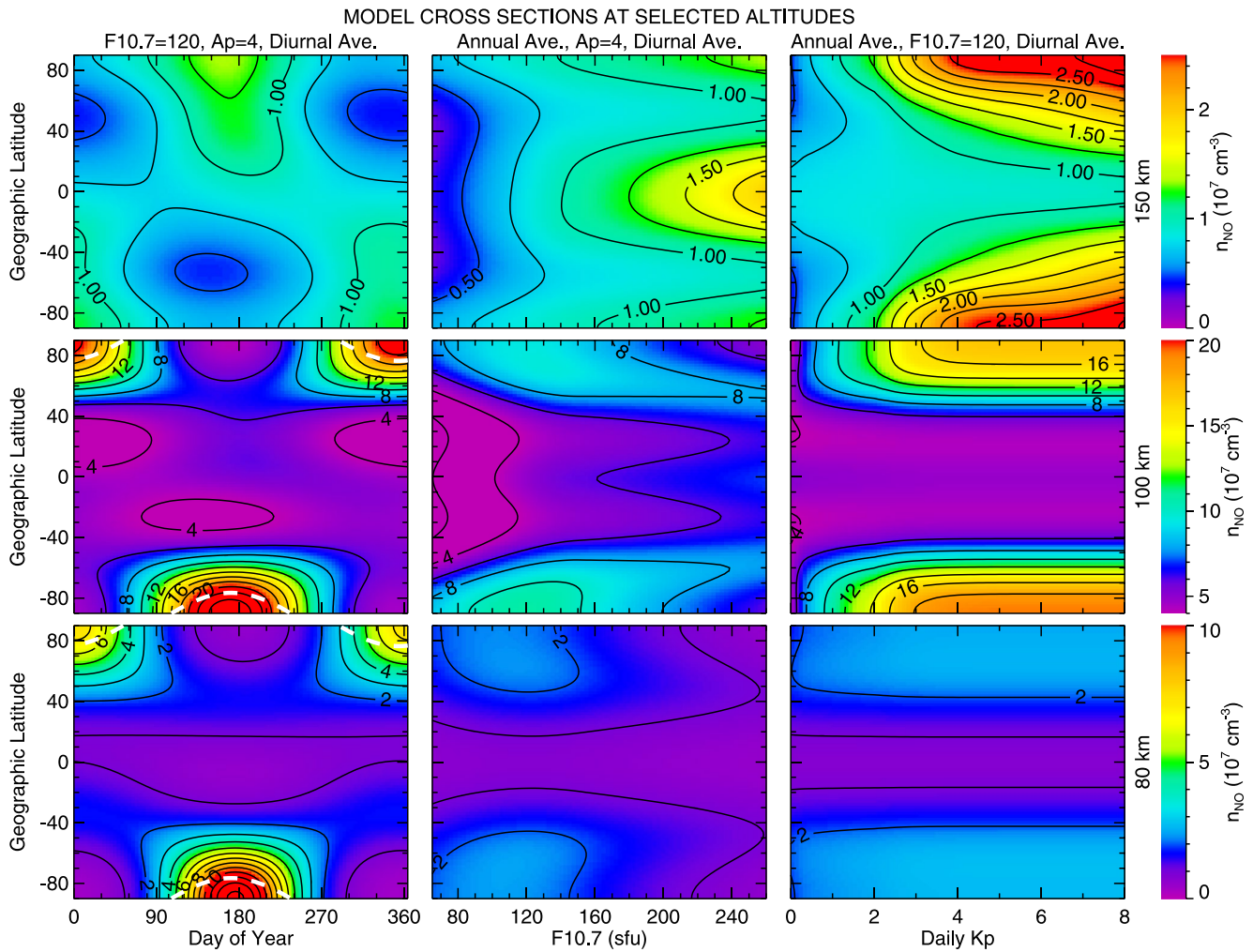
Figure 5. (Left) MSIS 2.1 nitric oxide (NO) density as a function of latitude and day of year, for solar moderate ( \overline{F}_{10.7} = 120 sfu) and geomagnetically quiet ( A_p = 4 ) conditions. In the lower two panels, the dashed white line marks the approximate solar terminator (solar zenith angle = 100^\circ ) at noon, which is the boundary of the polar night region. (Center) Same, but as a function of latitude and \overline{F}_{10.7} , for annually averaged, geomagnetically quiet ( A_p = 4 ) conditions. (Right) Same, but as a function of latitude and daily K_p for annually averaged, solar moderate ( \overline{F}_{10.7} = 120 sfu) conditions. Results are shown at three altitudes: (Top) 150 km, (middle) 100 km, and (bottom) 80 km. In all cases, the results are diurnal averages. The contour intervals and color range are different for each altitude, as indicated by the contour labels and color scales to the right.
