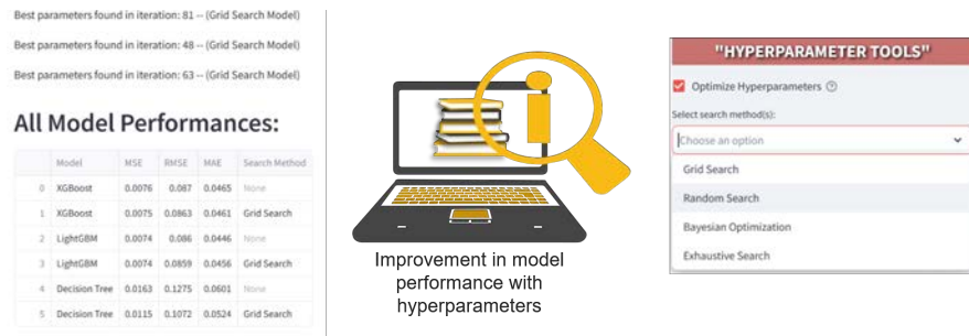
FIGURE 7. Hyperparameters Tuning.
