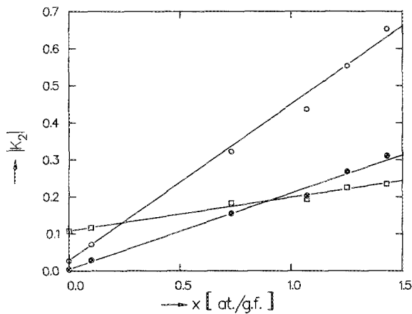
FIG. 12. Oscillator amplitude |K_{2i}| of those paramagnetic transitions sensitive to the bismuth concentration x in the LPE-grown \text{Y}_{3-x}\text{Bi}_x\text{Fe}_5\text{O}_{12} films whose dielectric tensor components are depicted in the Figs. 10 and 11; full circles: transition at h\nu_i \approx 2.63 eV; open circles: transition at h\nu_i \approx 3.40 eV, and open squares: transition at h\nu_i \approx 4.45 eV (see Table IV) (see Ref. 23). Experimental data at 295 K.
