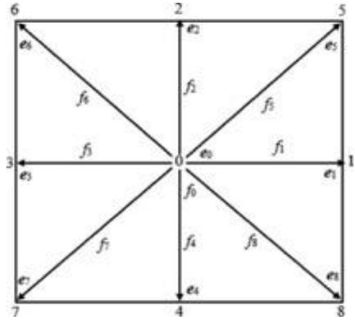
Fig. 2 Lattice structure for d2q9 model
