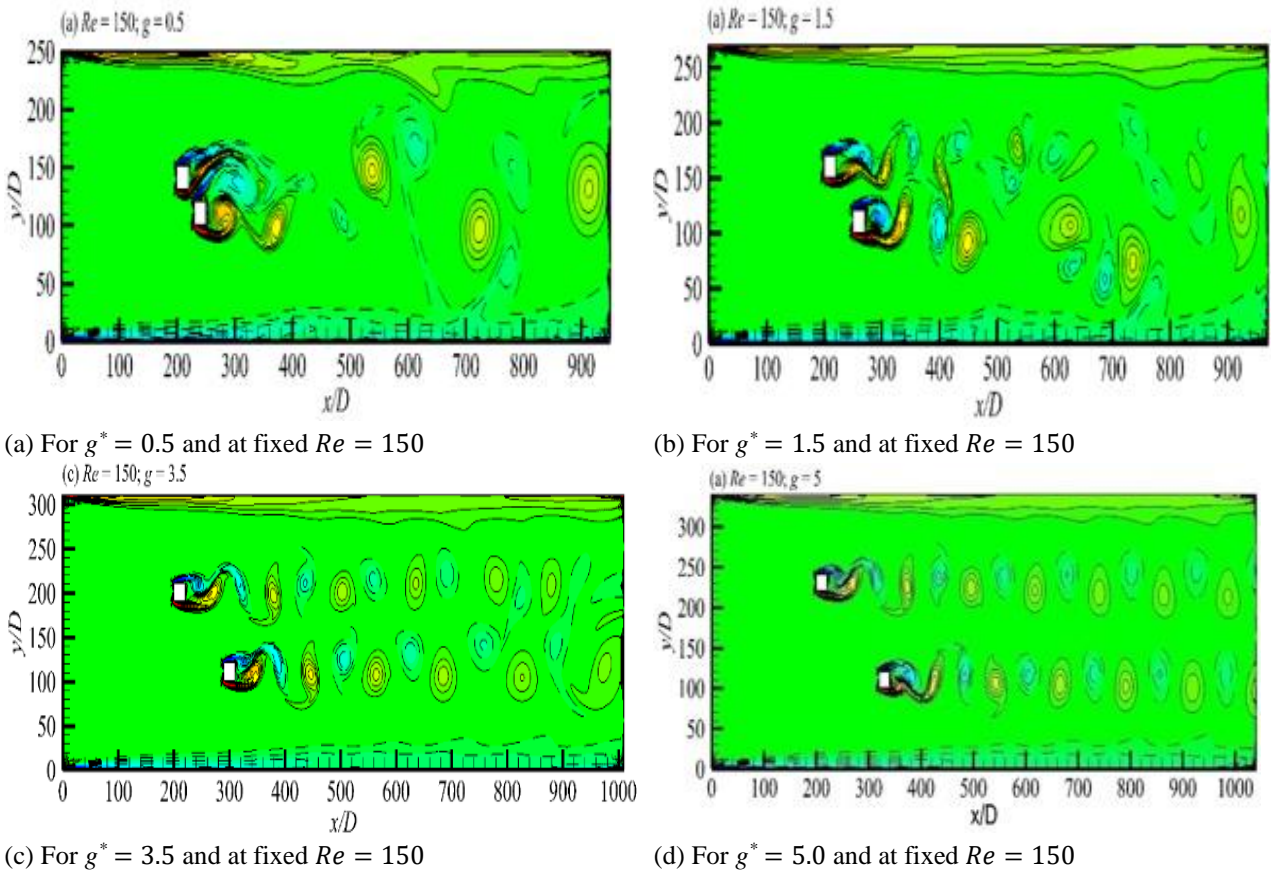
Fig. 6 Visualization of vorticity contours in the flow around two square cylinders positioned off-center, with variations in their configuration of g^* and at fixed Re = 150
