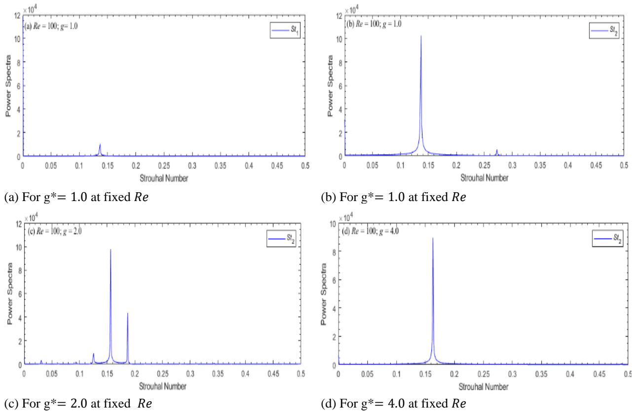
Fig. 14 Examination of power spectra and lift coefficient studies at various g^* at a fixed Re = 100
