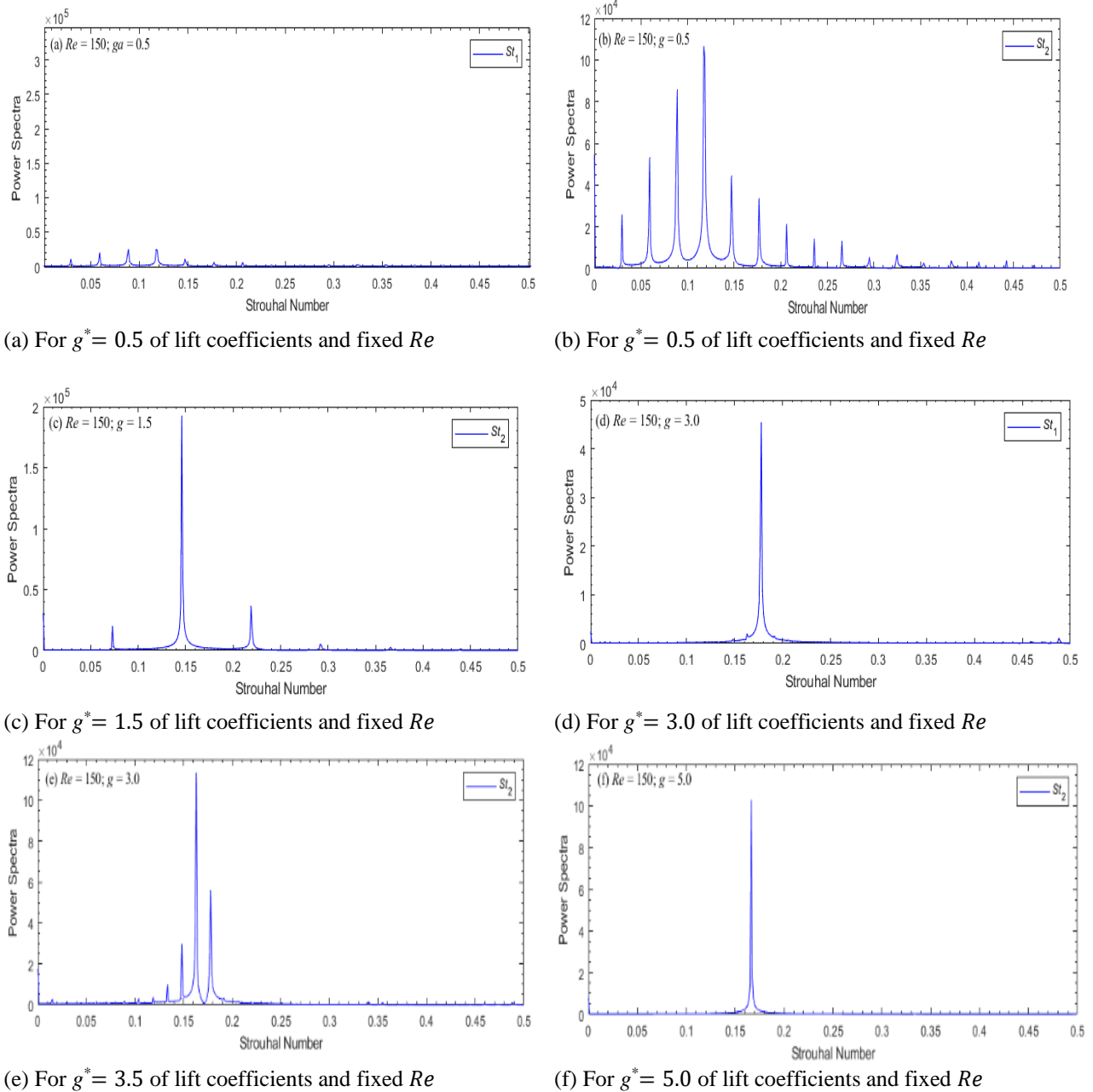
Fig. 8 Power spectra analysis of coefficients lift at varying g^* and at fixed Re = 150
