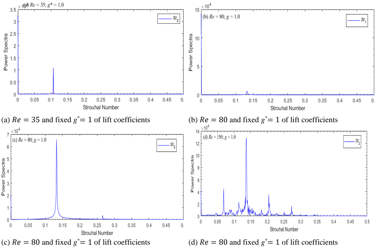
Fig. 5 Analyzing the power spectra at various values of Re and fixed g^* = 1 of lift coefficients
