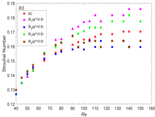
(c) St along with various spacing ratio from 0.5 to 5
