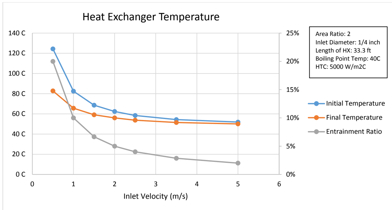
Figure 44: Inlet velocity vs heat exchanger temperatures, performance curve from CFD
