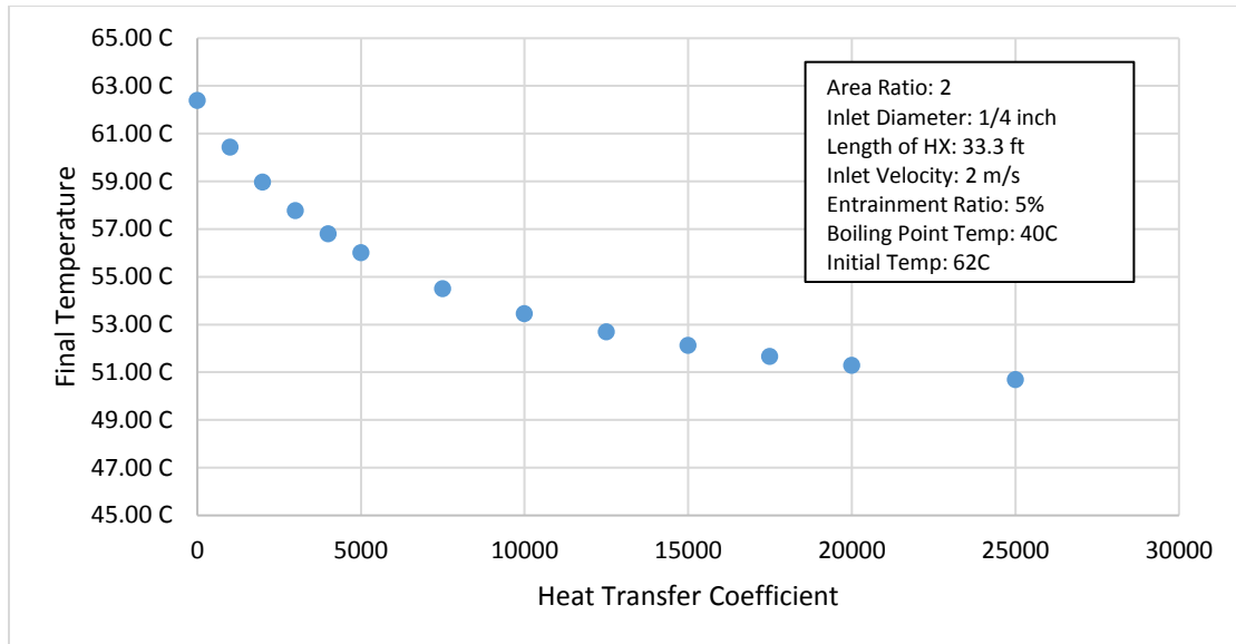
Figure 42: Final temperature vs heat transfer coefficient, performance curve from CFD
