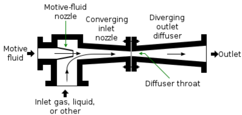
Figure 16: Operation of Liquid Jet Ejector [57].
