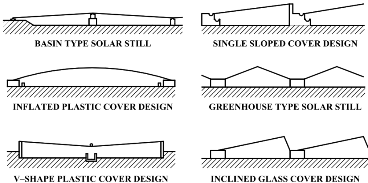
Figure 10: Common designs of solar stills [3].
