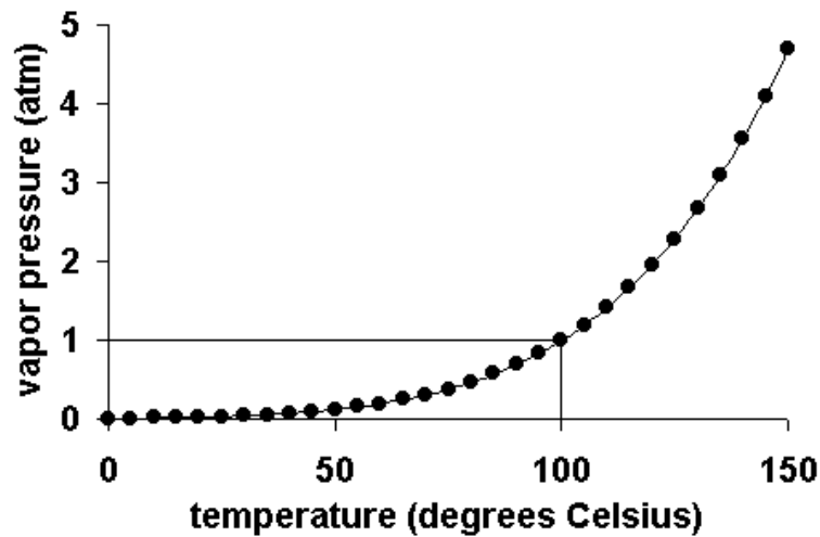
Figure 17: Saturated vapor pressure of water at different temperatures [51].
