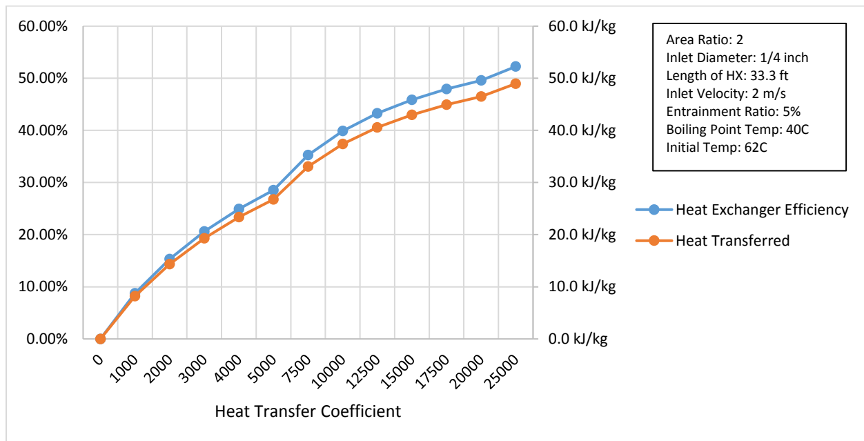
Figure 43: Heat transfer coefficient effect on heat exchanger behavior, performance curve from
