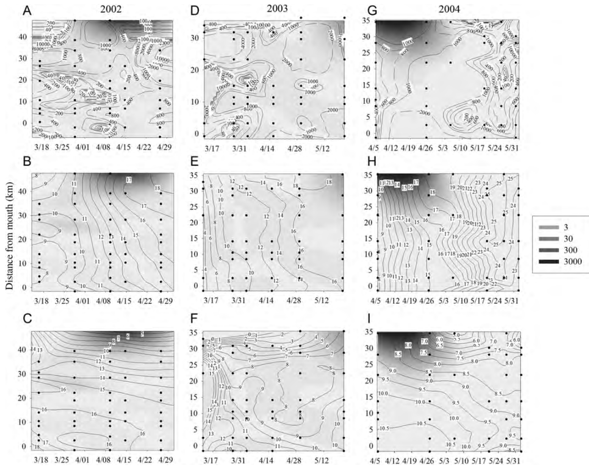
Fig. 4. Abundance of M. rubrum (gray scale contours, all plots) with cryptophyte algae (cells mL -1 ; A , D and G ), temperature (°C; B , E and H ) and salinity (PSU; C , F and I ) overlaid as lined contours, during spring in the Patuxent River (2002–2004). Numbers on plots refer to levels of cryptophytes, salinity or temperature along line contours. Gray-scale legend indicates M. rubrum abundance in cells mL -1 . X-axis indicates distance from mouth of river (km) and black dots indicate sampling stations.
