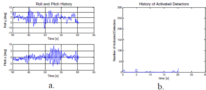
Figure 6-Validation data set [14]
