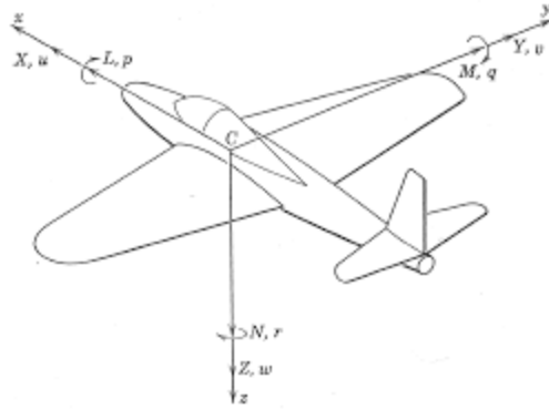
Figure 8-Airplane coordinate system
