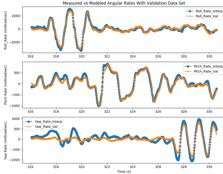
Figure 70-Fitted output under nominal conditions for run MIMO_04_05_2020__18_19_57
