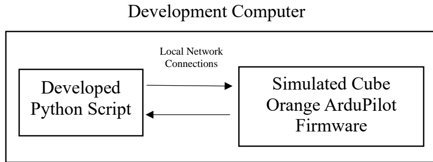
Figure 17-SITL diagram
