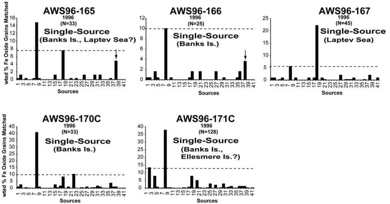
Figure 5. Source matches for five floes sampled in the Chukchi Borderland area in 1996. Arrows indicate the local Chukchi Sea source.
