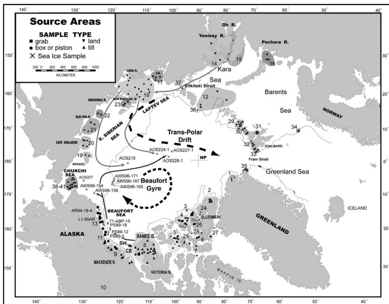
Figure 1. The sea ice sample locations and the general sea ice circulation (bold dashed arrows) in the Arctic Ocean. The proposed drift trajectories (gray arrows) shown are for the general areas where floes were sampled and are based both on the Fe oxide grain sources and buoy backtrajectories with known or general surface currents. Samples from Sachs Harbor (SH) are too close together to show. The Cape Bathurst (CB) Polynya generally occurs in the coastal waters between Banks Island and the Mackenzie Delta.
