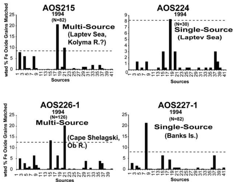
Figure 6. Source matches for four floes sampled in the west-central Arctic in 1994.
