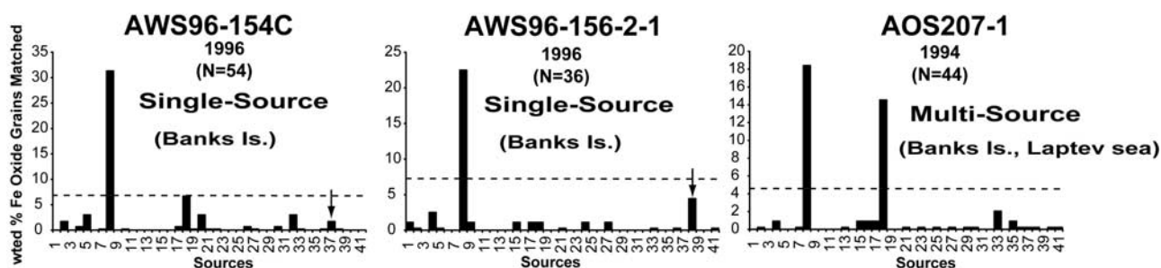
Figure 4. Source matches for three floes sampled in the northern Chukchi Sea. Arrows indicate the local Chukchi Sea source.
