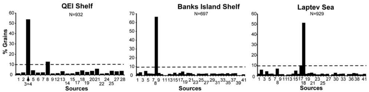
Figure 2. Matches of grains from three important source areas to all other source areas in the circum-Arctic. N is the number of grains matched, and the dashed line indicates the minimum percentage of grains for a match, which is a function of N (see text for discussion).
