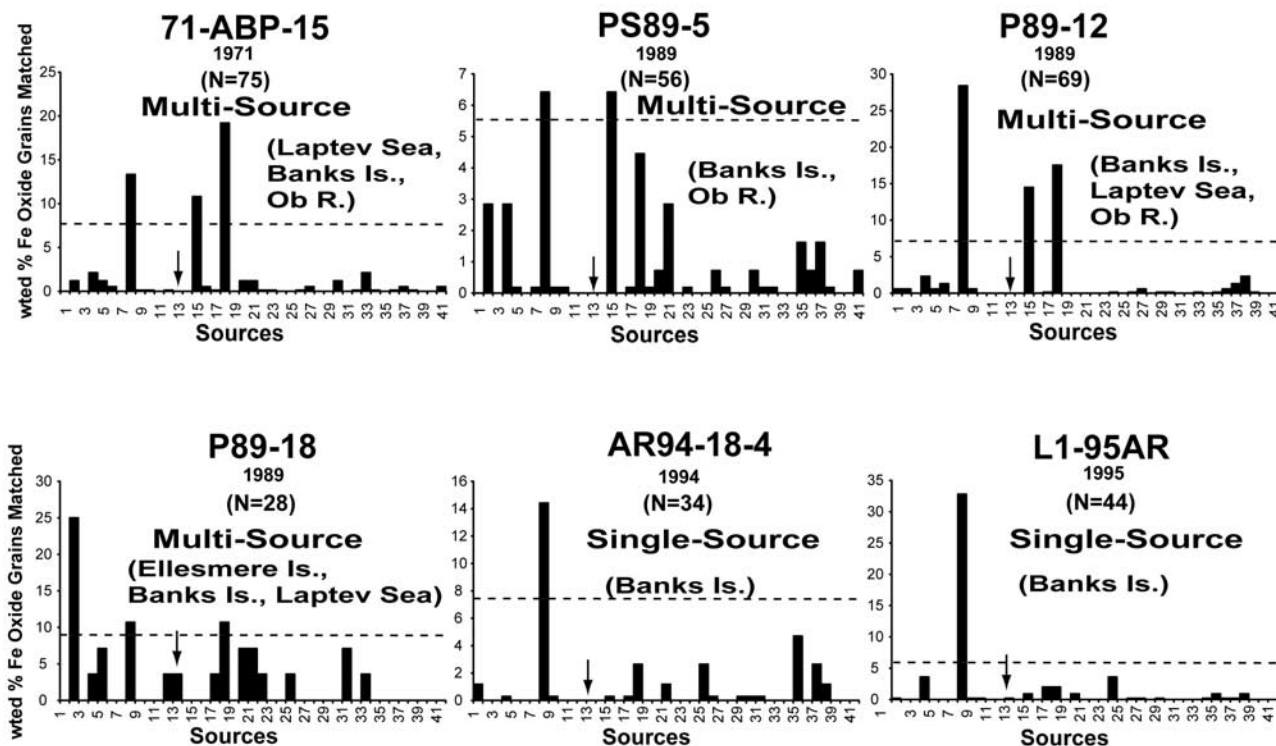
Figure 3. The weighted percent of Fe oxide grains from sea ice floes in the Beaufort Sea matched to circum-Arctic source areas. Arrows show the local northern Alaska shelf source area (source area 13). The Banks Island source (source area 8) is significant in every sample.
