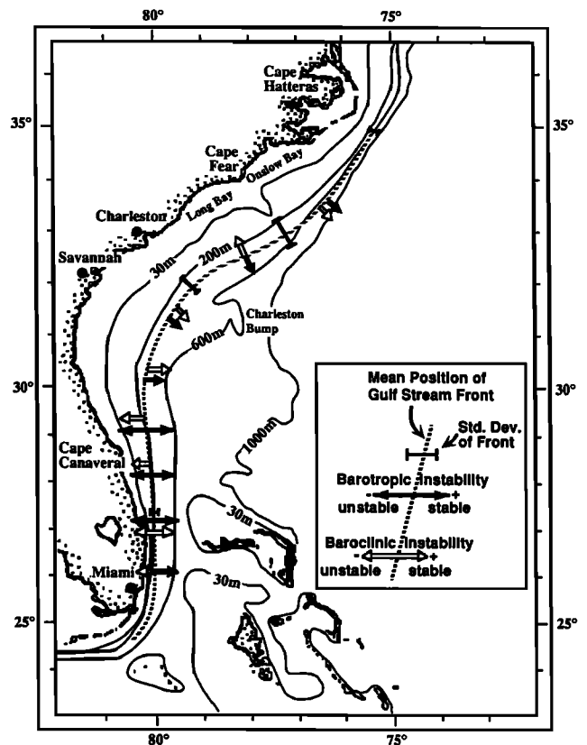
Fig. 6. Estimates of energy transfer terms \overline{u'v'} \partial\bar{v}/\partial x (negative or onshore for barotropic instability), \overline{u'\rho'} \partial\bar{\rho}/\partial x |\partial\bar{\rho}/\partial z|^{-1} (negative or onshore for baroclinic instability), term estimates, and data sources given in Table 1 (frontal positions from Figures 1 and 2 of Hood and Bane [1983]).
