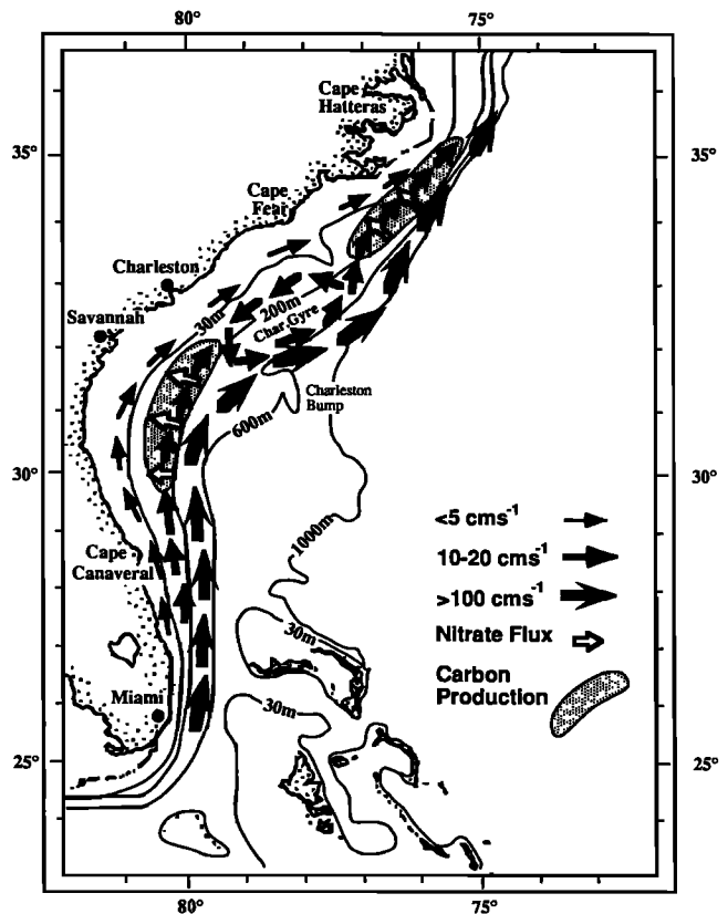
Fig. 8a. Characterization of mean circulation, onshore nitrate flux, and sites of potential Gulf Stream-induced new carbon production in the SAB during winter and spring conditions.
