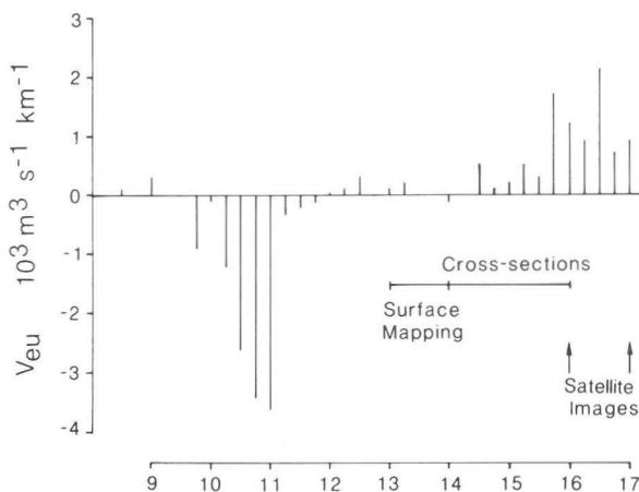
Fig. 4. Upwelling indices calculated for 43°N 11°W for the period 9–17 April 1981.
