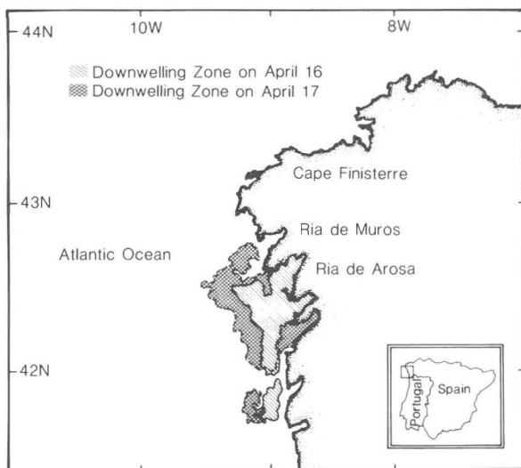
Figure 14. Demarcation of warm-water region indicated by infrared data from NOAA-6 satellite. The data came from processed images at the Image of Processing Laboratory at Rosenstiel School of Marine and Atmospheric Sciences of the University of Miami. See Figure 4 for relationship in time to the hydrographic cruise data.
