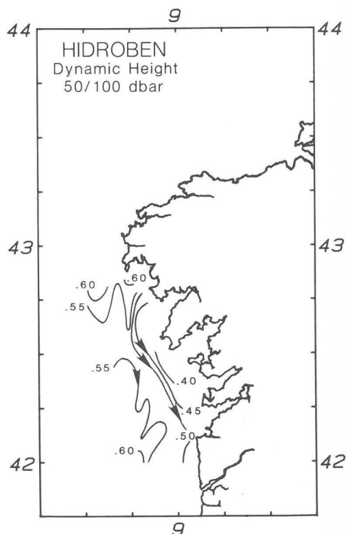
Figure 12. Dynamic height of the 50-dbar surface relative to the 100-dbar surface. Units are dynamic meters.
