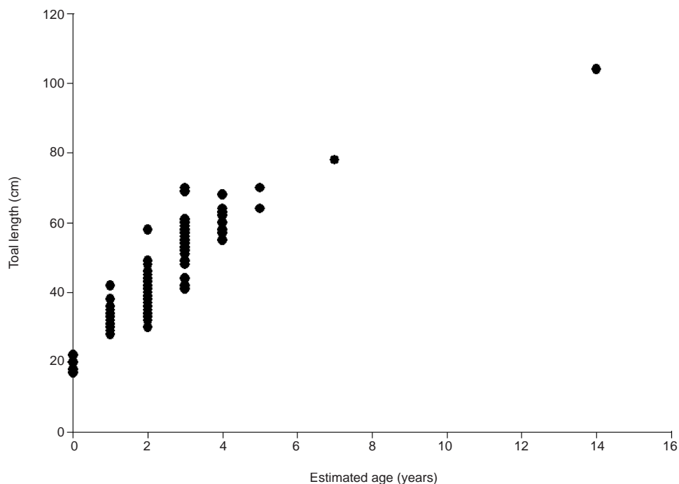
Figure 4: Size-at-age for the sample of Dissostichus eleginoides taken off South Georgia in January 2000.
