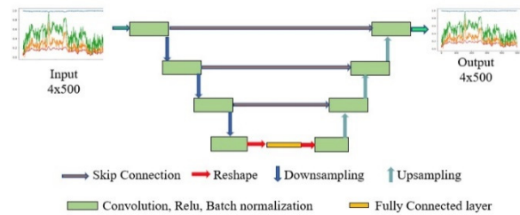
Figure 4: U-Net architecture for binary classification.
