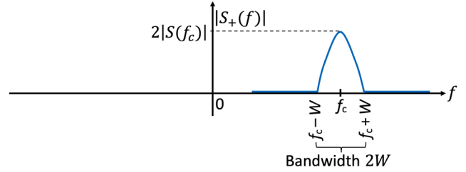
(b) Amplitude spectrum for pre-envelope signal s_+(t) .
