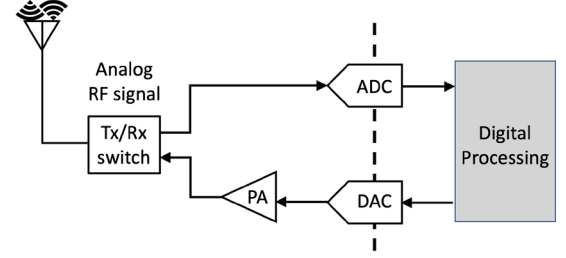
Fig. 6. Ideal architecture of a SDR. The ADC and DAC are performed on the RF signal, and a power amplifier (PA) is used on the transmit side to ensure desired RF transmit power level.
