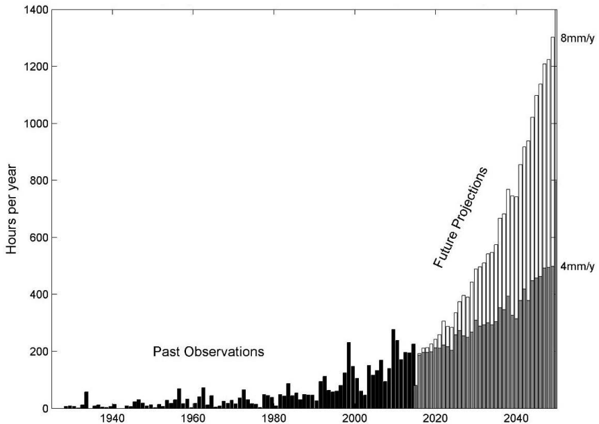
FIGURE 6. Hours per year that minor flooding starts in the streets of the historic Hague district of Norfolk, VA, when water level is ~1 ft (30 cm) above MHHW. Black bars are based on past observations of the tide gauge at Sewells Point; gray and white bars are estimated projections until 2050 for future SLR rates of 4 and 8 mm/y, respectively.
