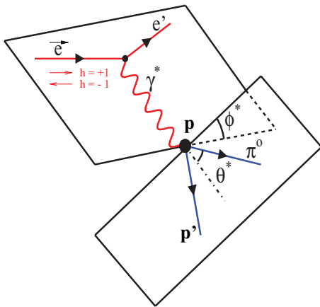
FIG. 1. (Color online) Schematic diagram of \pi^0 -nucleon electroproduction. \vec{e} represents the incident polarized electron, e' is the outgoing electron, \gamma^* is the virtual photon, and p and p' are the nucleon in the initial and final states, respectively.
