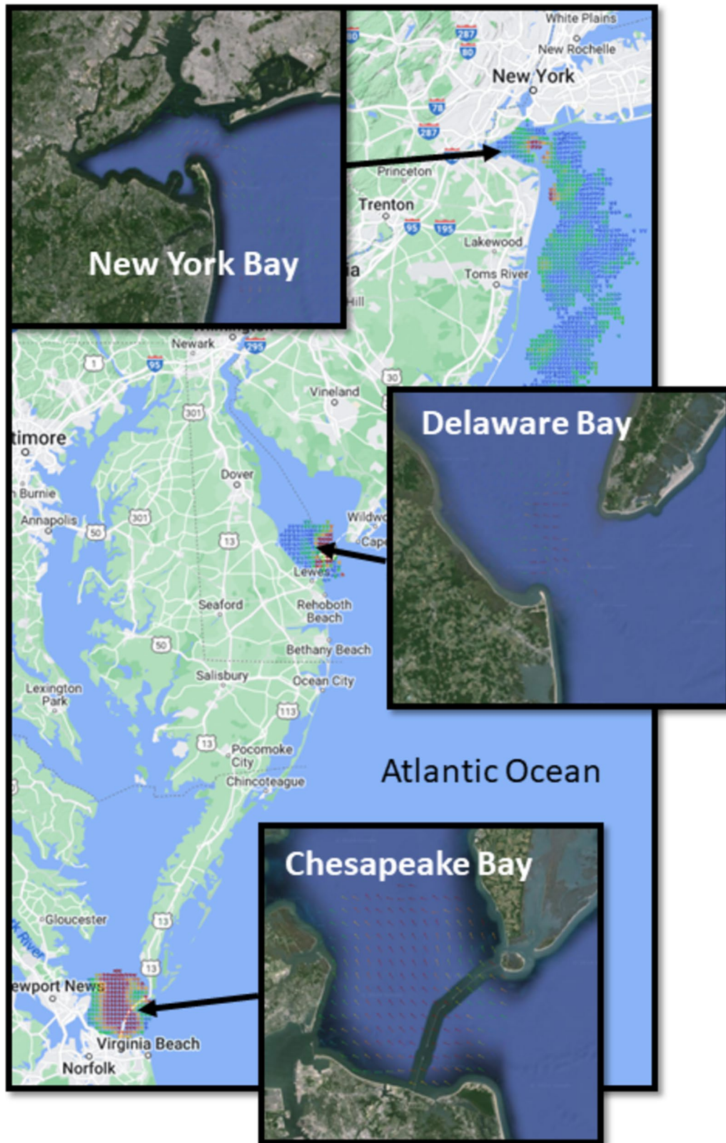
Fig. 1 A map of the study area and the CODAR 2 km data for the three locations: Chesapeake Bay (CB), Delaware Bay (DB) and New York Bay (NB). The surface currents shown here are examples during arbitrary day, for mean currents over the study period see Fig. 2
