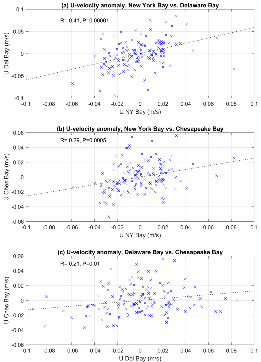
Fig. 4 Scatter plots and correlations between the detrended flows of the three bays. Statistical significance of the correlation coefficients range between 99% (DB vs. CB; Fig. 4c) and 99.999% (DB vs. NB)
