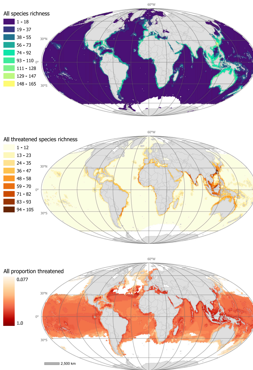
Figure 5. Global chondrichthyan richness and threat
