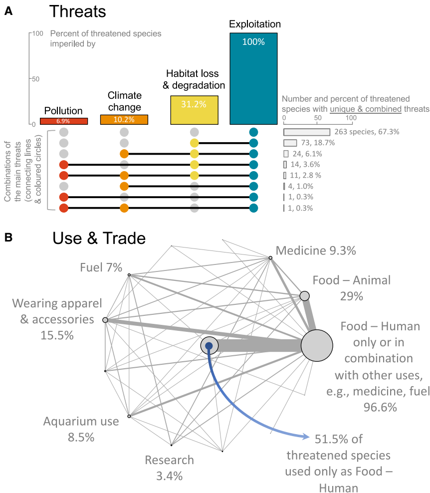
Figure 3. Threats to chondrichthyans and the use and trade of the species threatened by overexploitation
