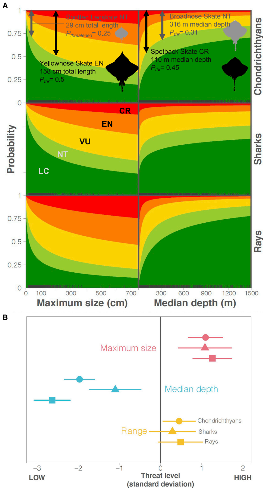
Figure 4. Global trait models of chondrichthyan extinction risk
