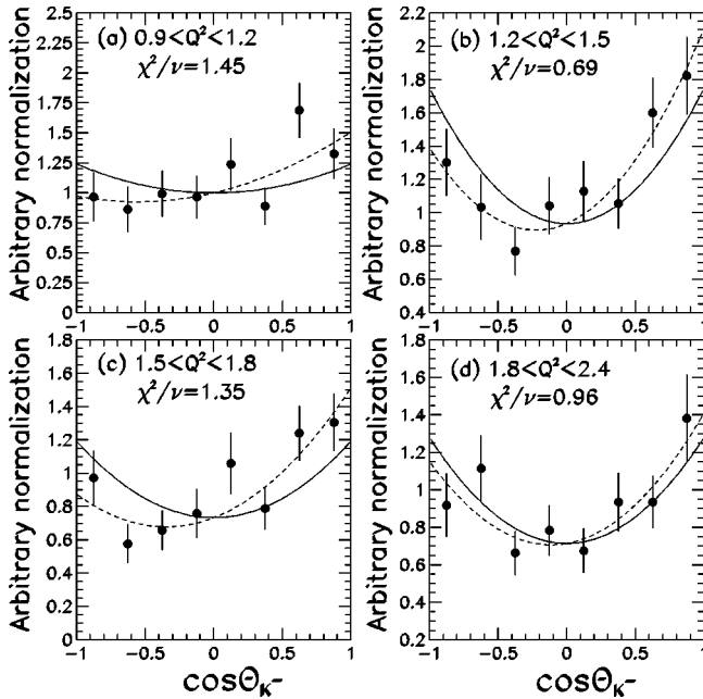
FIG. 9. The \Lambda(1520)\cos \theta_{K-} decay angular distribution for four regions of Q^2 . These distributions are averaged over the region of W from threshold to 2.43 GeV. The error bars are statistical uncertainties only. The plotted curves are explained in the text.
