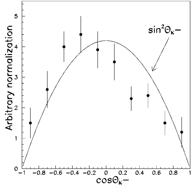
FIG. 10. The \Lambda(1520) photoproduction decay angular distribution published previously in Ref. [1]. The \sin^2 \theta_{K-} curve included with these data is the expected distribution if the \Lambda(1520) decay is entirely due to the m_z = \pm \frac{3}{2} spin projection, and is not a fit to the data.
