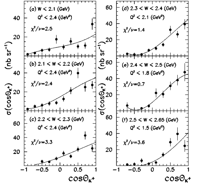
FIG. 4. The \cos \theta_{K^+} differential cross section distributions for six regions of W . The error bars are statistical uncertainties only. The solid lines represent Legendre polynomial fits that are described in the text. The lower limit Q^2 = 0.9 GeV 2 is used for all six distributions.
