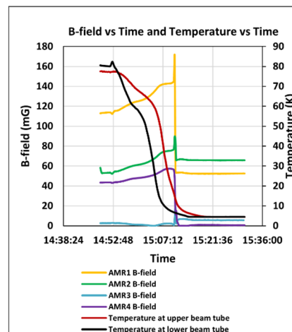
Figure 7: Magnetic field vs. time and temperature vs. time.
