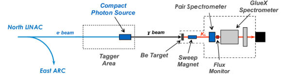
Figure 1: Schematic view of Hall D beamline on the way e \rightarrow \gamma \rightarrow K_L . Electrons first hit the copper radiator inside the Compact Photon Source (CPS). Then photons illuminate the Be target, and finally, neutral kaons hit the \text{LH}_2/\text{LD}_2 cryogenic target. Beam goes from left to right [1].
