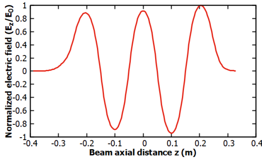
Figure 3: 1 D field map used for Nb 3 Sn cryomodule in the computer simulation.
