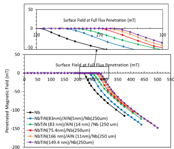
Figure 7: Full flux penetration detected by the center Hall probe through layered niobium comparing with the bare niobium substrate at 2.00 K.
