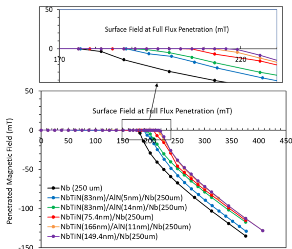
Figure 6: Full flux penetration detected by the centre Hall probe through the layered niobium comparing with the bare niobium substrate at 4.35 K.
