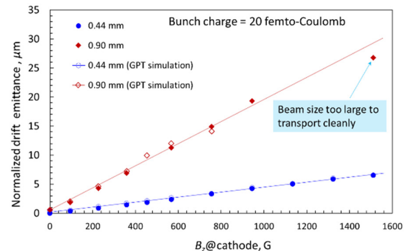
Figure 4: Measured and GPT simulation results of drift emittance versus cathode solenoid field for two laser spot sizes.
