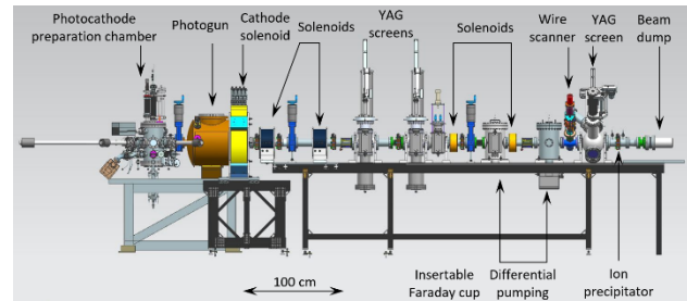
Figure 1: Illustration of main components of the magnetized electron beamline.
