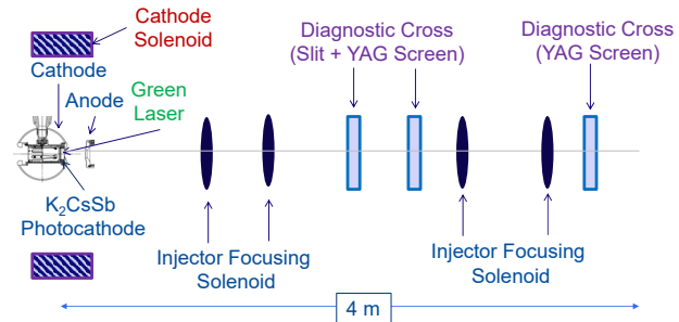
Figure 1: The diagnostic beamline.
