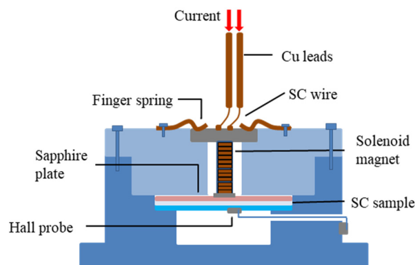
Figure 1: Schematic cross section of experimental setup.
