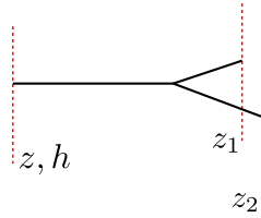
Fig. 5. Graphical representation of the projection (44) of color dipole on the E -eigenfunction. Dotted lines represent the Wilson lines and all the coordinates correspond to the transverse 2-dimensional space.
