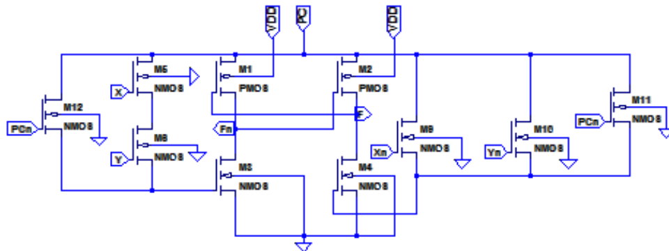
Figure 16: IDPAL AND/NAND Logic Gate – Schematic
