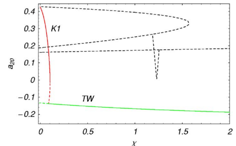
FIG. 2. Bifurcation diagram of a_2^0 as a function of anisotropy \chi at parameter values Pe=3 , \tilde{a}=1 , and N=5.5 . The shear response is K_1 for zero anisotropy \chi=0 . As \chi increases, the K_1 attractor collapses to a tumbling/wagging (TW). In a very narrow band of \chi , the K_1 and TW attractors coexist.
