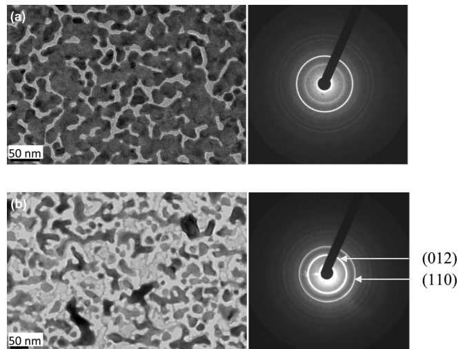
FIG. 1. HRTEM images and diffraction pattern of as-deposited 5 nm thick Bi film (a) and laser annealed sample at laser fluence of 2.4 mJ/cm 2 operated at 1 kHz repetition rate (b). Laser annealing causes some agglomeration of the as-deposited islands and an increase of voids. The diffraction patterns are characteristic of the bulk hexagonal unit cell, indicating no structural phase transition occurring during annealing. The ring intensities change by annealing indicating changes in film orientation.
