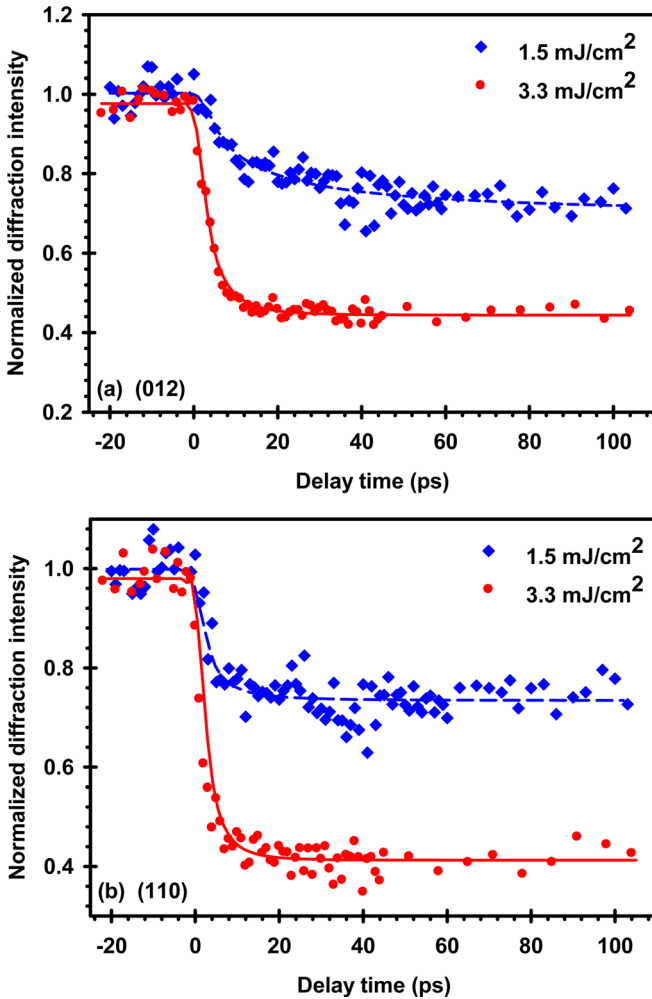
FIG. 2. (Color online) Time evolution of Bragg peak normalized intensity. (a) For the (012) planes, the decay time \tau is 11.2 and 4.1 ps for laser fluence of 1.5 and 3.3 mJ/cm 2 , respectively. (b) For the (110) planes, \tau is 4.3 and 3.1 ps for laser fluence of 1.5 and 3.3 mJ/cm 2 , respectively. Anisotropy in the decay time of the (012) and (110) peaks indicates different lattice excitation mechanisms that is dependent on crystal direction.
