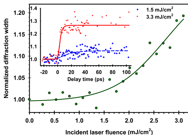
FIG. 3. (Color online) Diffraction width of the (012) Bragg peak normalized to that without laser heating taken at delay time 41 ps for different laser fluences. Inset is time evolution of normalized Bragg peak width at two different laser fluences.
