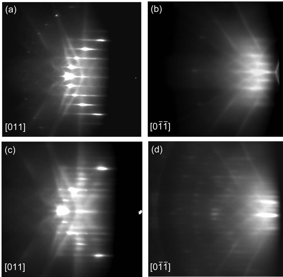
FIG. 1. [(a) and (b)] RHEED patterns of Si(100)-(2 \times 1) surface before In deposition taken along the [011] and [0 \bar{1}\bar{1} ] azimuths, respectively. [(c) and (d)] RHEED patterns of In(4 \times 3) grown on Si(100)-(2 \times 1) by femto-second PLD taken along the [011] and [0 \bar{1}\bar{1} ] azimuths, respectively. The laser was operated at a 2 Hz repetition rate with an energy density of 0.50 J/cm 2 on the In target.
